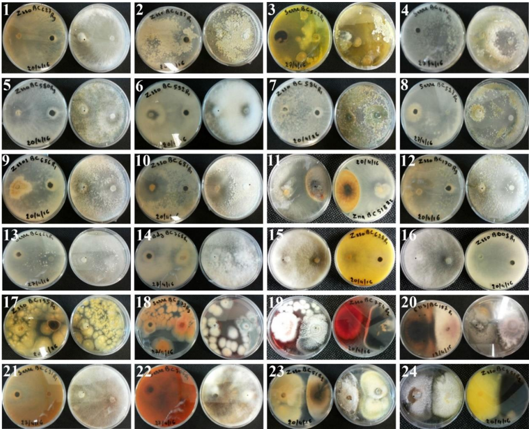
Figure 4: Dual culture of M. oryzae to evaluate its antagonism potential and systems. In these Petri dishes, the fungi M. oryzae is in black color and the other colors represent the bioagents. Using scale of the type of antagonism proposed by Scaufilaire et al. (2015), three different types of interaction between antagonists were observed viz /Antagonists touch each other; // : Presence of inhibition zone. For three BCAs, a zone of inhibition appears between the candidate and the pathogen, including Penicillium (BC754), Fusarium (BC187), and Cladosporium (BC51); A: colonization of the pathogen. Other candidate BCAs colonized the mycelium of the pathogen mainly by Trichoderma and constitutes the best candidate. Another type of antagononism was observed between BC851 and M. oryzae touched each other without a zone of inhibition.
