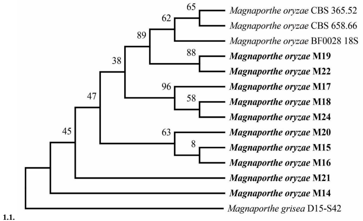
Figure 3: Phylogenetic tree inferred from a Maximum Parsimony analysis of taxa based on analyses of a concatenated alignment of ITS sequence of rADN of 14 strains representing the genus of Magnaporthe from suthern of Mali.
